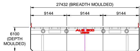
END ELEVATION - STERN END
